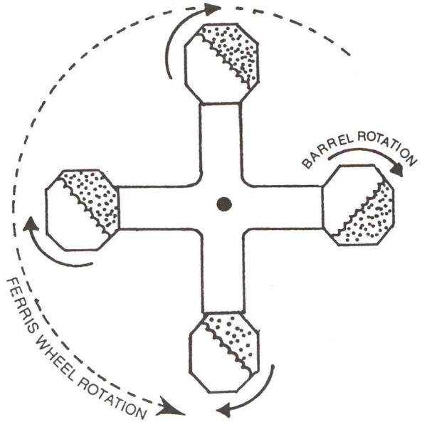
FIG. 18 HIGH ENERGY BARREL
