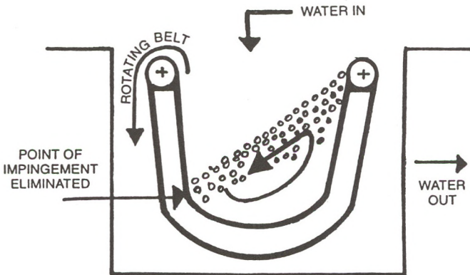
FIG. 20 ROLL BURNISHING
