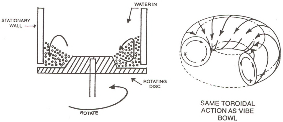
FIG. 19 HIGH ENERGY DISC
